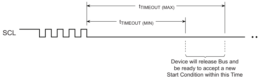
Figure 10-2. SMBus Timeout
